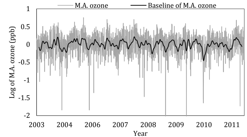
Constructing M.A. ozone for C31 (Frisco)
