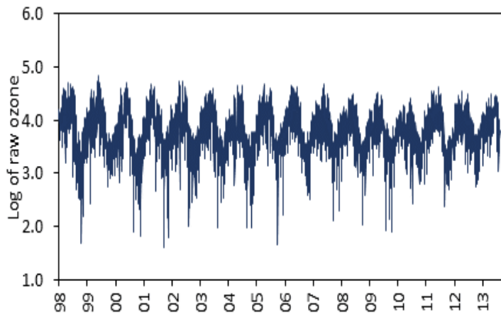
Log-transformed raw ozone time series
