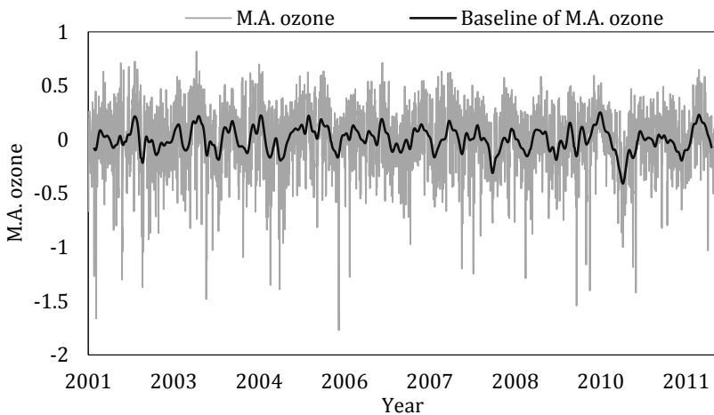
Constructing M.A. ozone for C56 (Denton)
